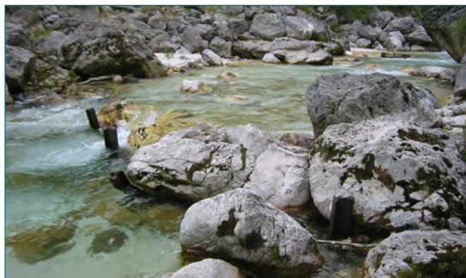
Bed and bank stabilization on the Soča, using steel pins
