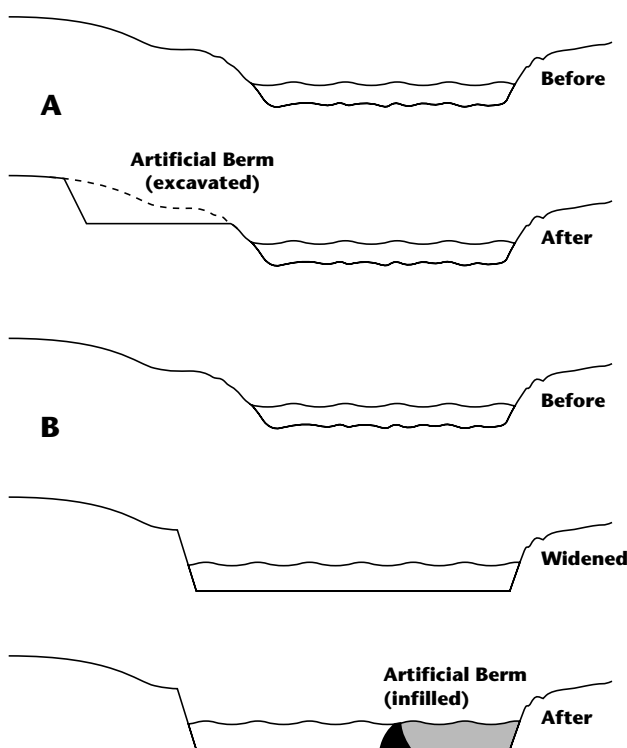
Figure I1 Artificial two-stage channel – berm formation through: A - bank excavation B - channel infill
