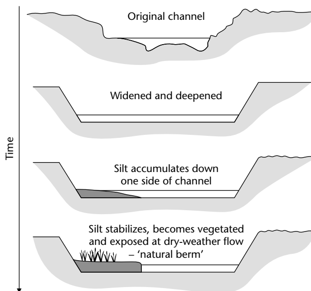
Figure E4 Cross-sections showing formation of 'natural berm' following recovery from channel over-widening
